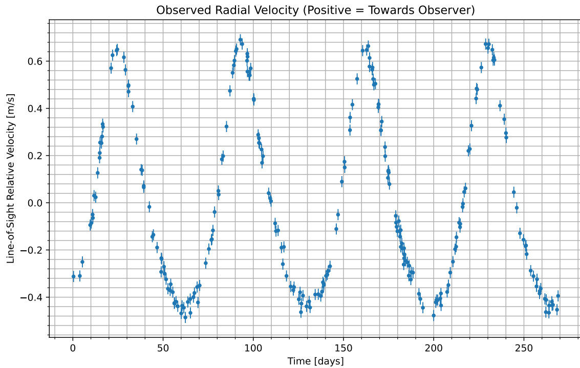
Figure 1: We have isolated the radial velocity of the host star due to the candidate planet. Data begins at UTC 2095-06-27/18:49. Positive values indicate the velocity at which the star is moving towards us; negative indicate the velocity at which it is moving away.
