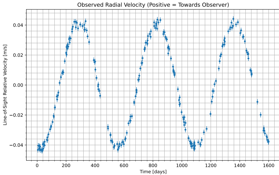
Figure 1: We have isolated the radial velocity of the host star due to the candidate planet. Data begins at UTC 2086-12-11/04:28. Positive values indicate the velocity at which the star is moving towards us; negative indicate the velocity at which it is moving away.
