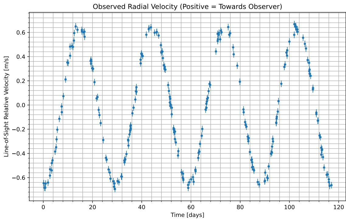
Figure 1: We have isolated the radial velocity of the host star due to the candidate planet. Data begins at UTC 2087-03-01/13:39. Positive values indicate the velocity at which the star is moving towards us; negative indicate the velocity at which it is moving away.
