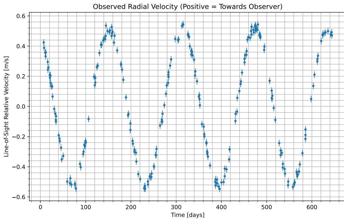
Figure 1: We have isolated the radial velocity of the host star due to the candidate planet. Data begins at UTC 2092-09-18/09:12. Positive values indicate the velocity at which the star is moving towards us; negative indicate the velocity at which it is moving away.
