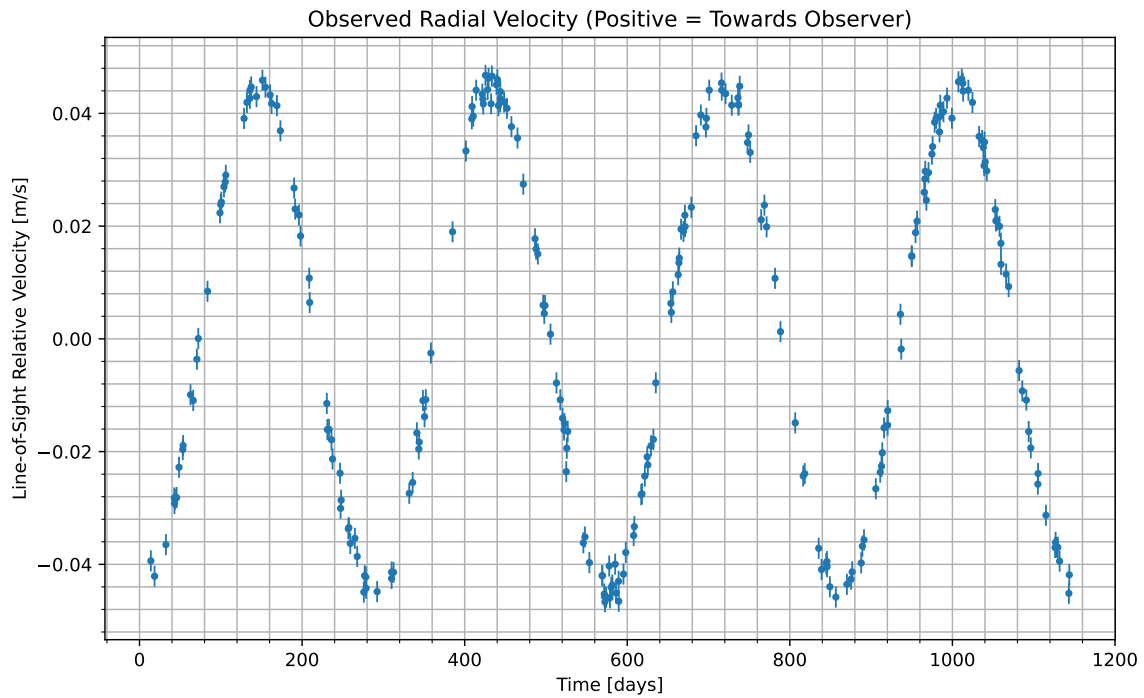
Figure 1: We have isolated the radial velocity of the host star due to the candidate planet. Data begins at UTC 2076-05-29/14:54. Positive values indicate the velocity at which the star is moving towards us; negative indicate the velocity at which it is moving away.
