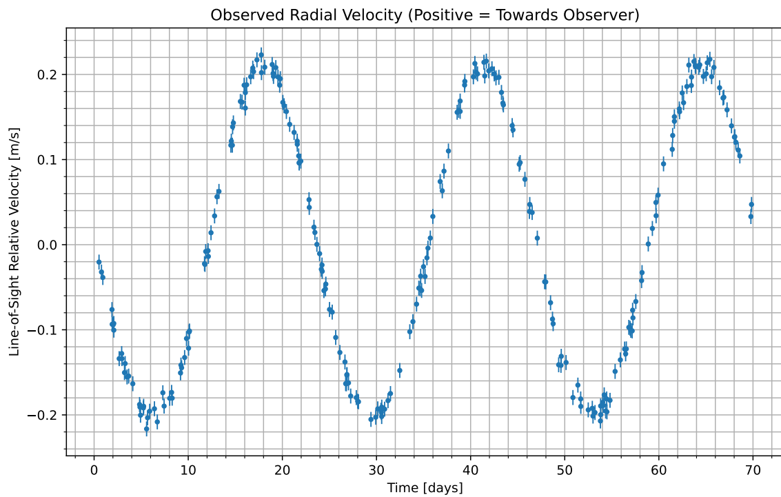
Figure 1: We have isolated the radial velocity of the host star due to the candidate planet. Data begins at UTC 2086-08-08/01:25. Positive values indicate the velocity at which the star is moving towards us; negative indicate the velocity at which it is moving away.
