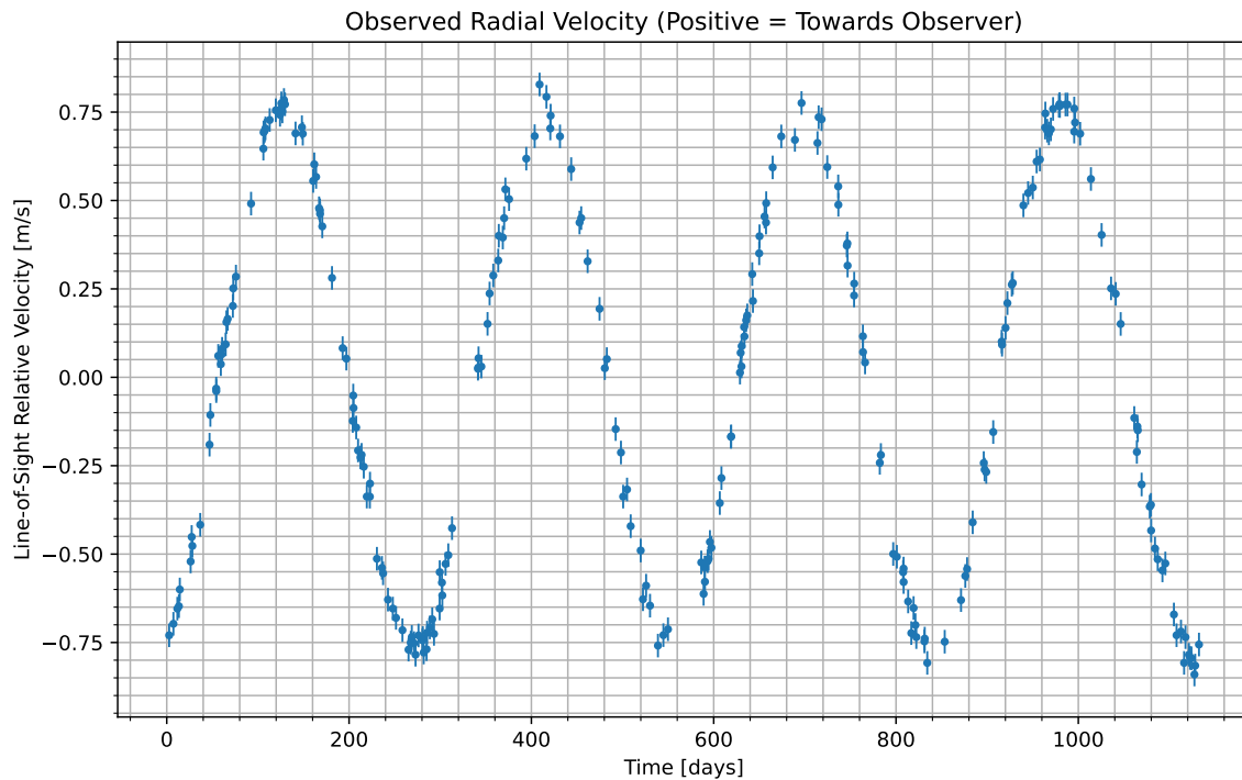
Figure 1: We have isolated the radial velocity of the host star due to the candidate planet. Data begins at UTC 2090-08-22/07:02. Positive values indicate the velocity at which the star is moving towards us; negative indicate the velocity at which it is moving away.
