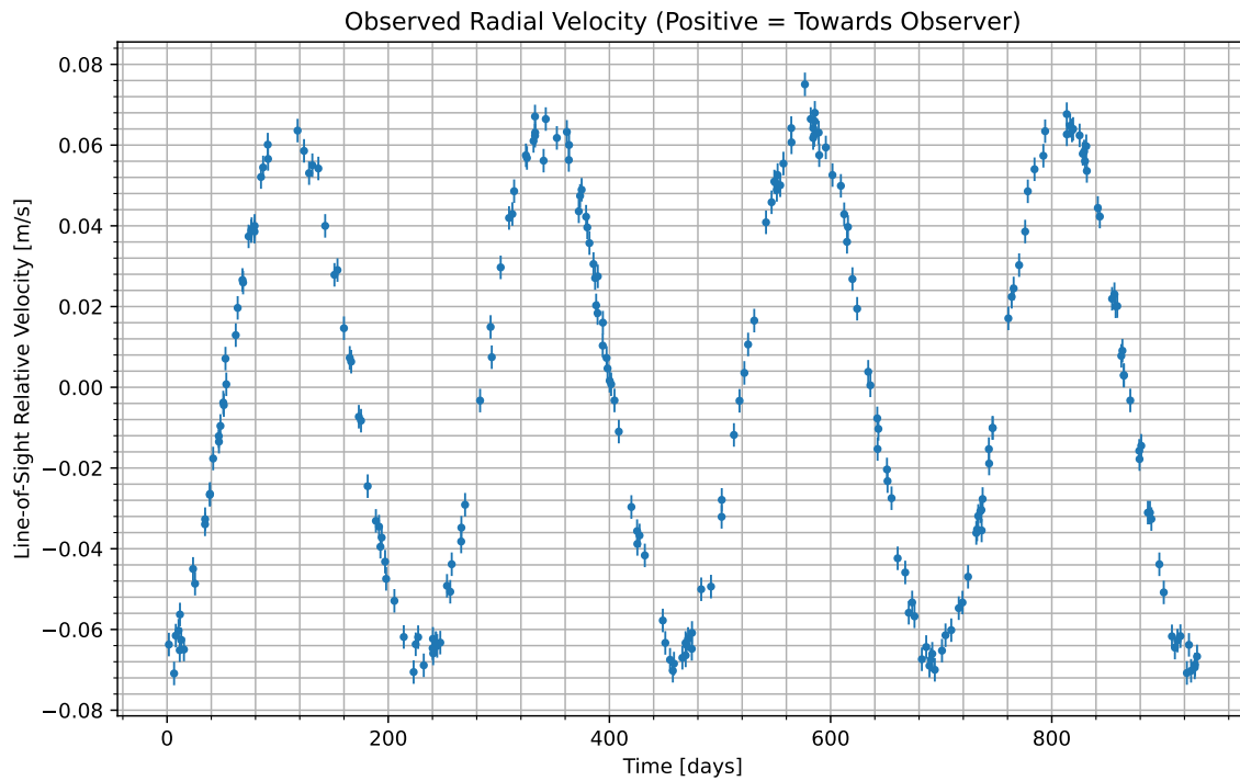
Figure 1: We have isolated the radial velocity of the host star due to the candidate planet. Data begins at UTC 2096-05-20/20:19. Positive values indicate the velocity at which the star is moving towards us; negative indicate the velocity at which it is moving away.
