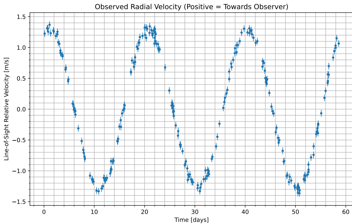
Figure 1: We have isolated the radial velocity of the host star due to the candidate planet. Data begins at UTC 2098-06-27/10:28. Positive values indicate the velocity at which the star is moving towards us; negative indicate the velocity at which it is moving away.
