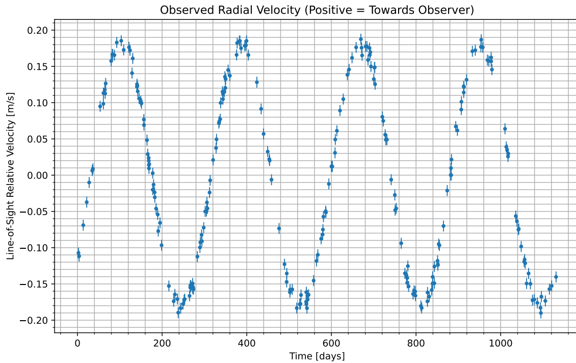
Figure 1: We have isolated the radial velocity of the host star due to the candidate planet. Data begins at UTC 2071-12-23/16:45. Positive values indicate the velocity at which the star is moving towards us; negative indicate the velocity at which it is moving away.
