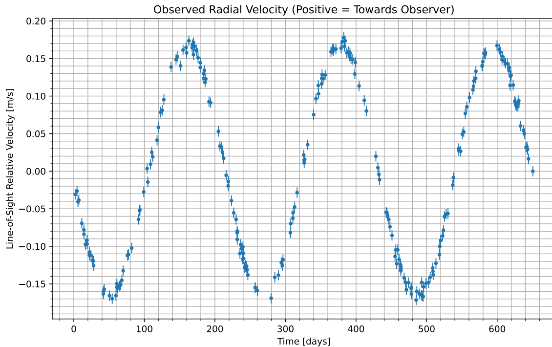
Figure 1: We have isolated the radial velocity of the host star due to the candidate planet. Data begins at UTC 2095-12-13/11:27. Positive values indicate the velocity at which the star is moving towards us; negative indicate the velocity at which it is moving away.
