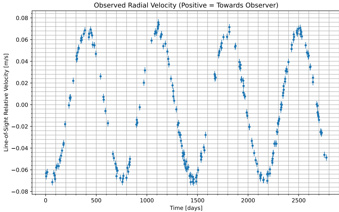
Figure 1: We have isolated the radial velocity of the host star due to the candidate planet. Data begins at UTC 2091-11-25/14:02. Positive values indicate the velocity at which the star is moving towards us; negative indicate the velocity at which it is moving away.
