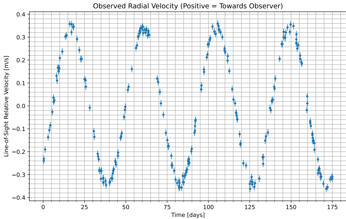
Figure 1: We have isolated the radial velocity of the host star due to the candidate planet. Data begins at UTC 2074-07-01/01:06. Positive values indicate the velocity at which the star is moving towards us; negative indicate the velocity at which it is moving away.
