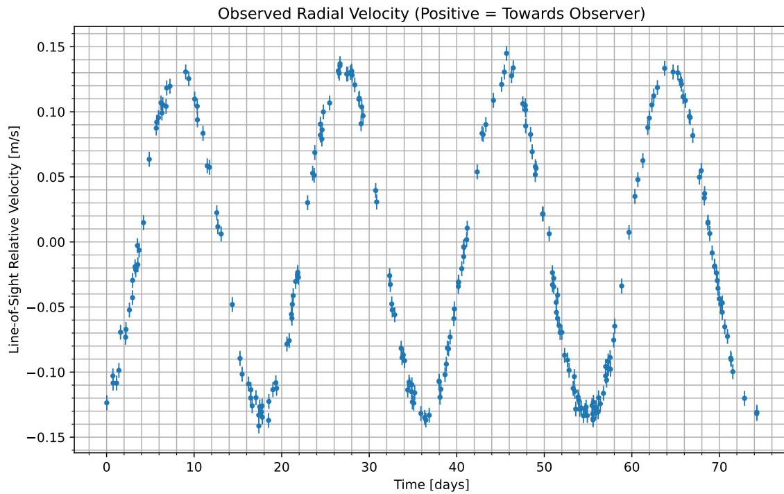
Figure 1: We have isolated the radial velocity of the host star due to the candidate planet. Data begins at UTC 2084-05-25/00:21. Positive values indicate the velocity at which the star is moving towards us; negative indicate the velocity at which it is moving away.
