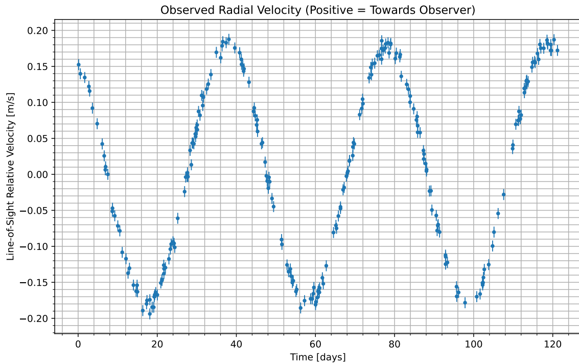
Figure 1: We have isolated the radial velocity of the host star due to the candidate planet. Data begins at UTC 2070-09-13/06:40. Positive values indicate the velocity at which the star is moving towards us; negative indicate the velocity at which it is moving away.
