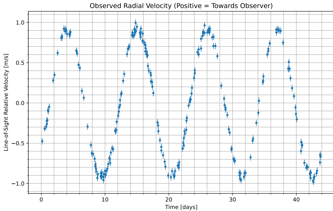
Figure 1: We have isolated the radial velocity of the host star due to the candidate planet. Data begins at UTC 2074-10-04/06:27. Positive values indicate the velocity at which the star is moving towards us; negative indicate the velocity at which it is moving away.
