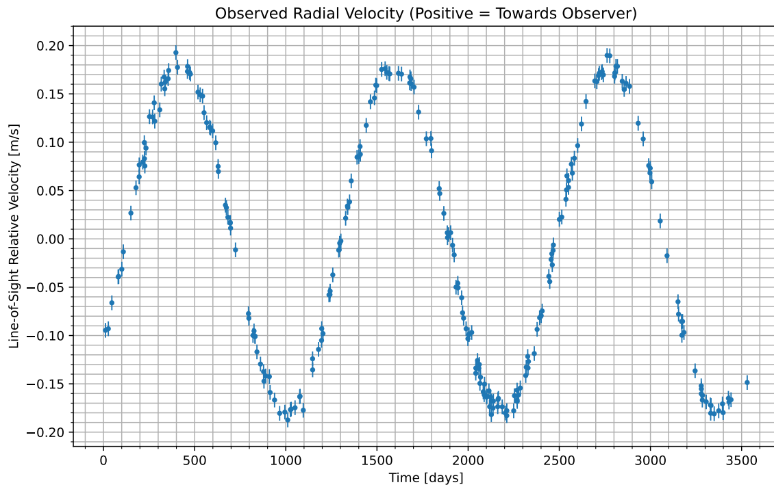
Figure 1: We have isolated the radial velocity of the host star due to the candidate planet. Data begins at UTC 2078-03-03/08:22. Positive values indicate the velocity at which the star is moving towards us; negative indicate the velocity at which it is moving away.
