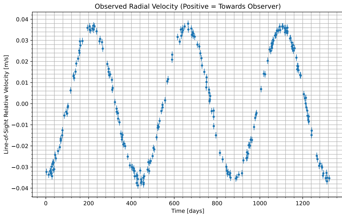
Figure 1: We have isolated the radial velocity of the host star due to the candidate planet. Data begins at UTC 2077-12-22/07:42. Positive values indicate the velocity at which the star is moving towards us; negative indicate the velocity at which it is moving away.
