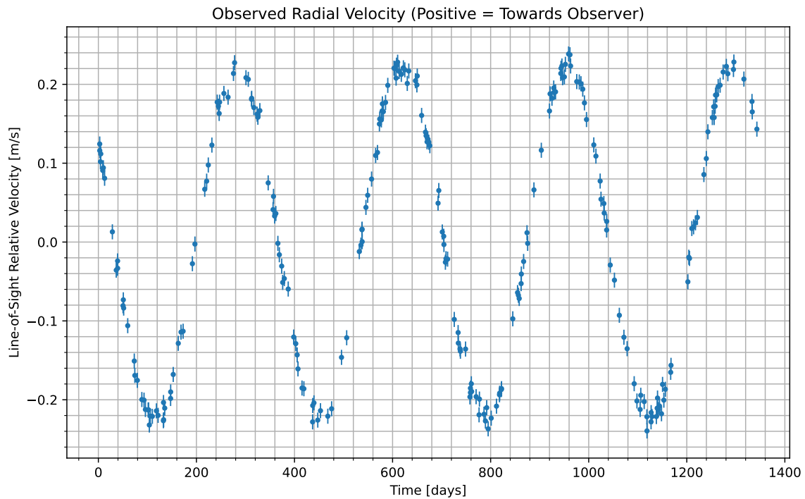
Figure 1: We have isolated the radial velocity of the host star due to the candidate planet. Data begins at UTC 2094-01-28/09:05. Positive values indicate the velocity at which the star is moving towards us; negative indicate the velocity at which it is moving away.
