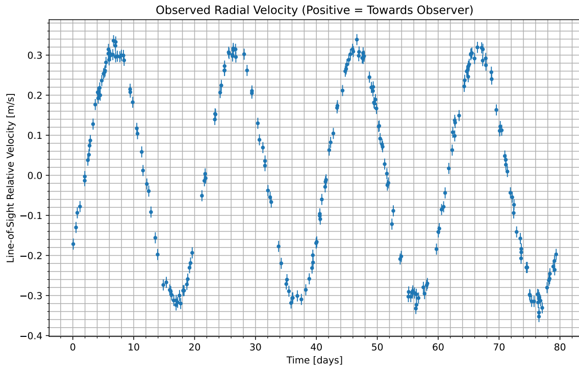
Figure 1: We have isolated the radial velocity of the host star due to the candidate planet. Data begins at UTC 2086-10-12/06:37. Positive values indicate the velocity at which the star is moving towards us; negative indicate the velocity at which it is moving away.
