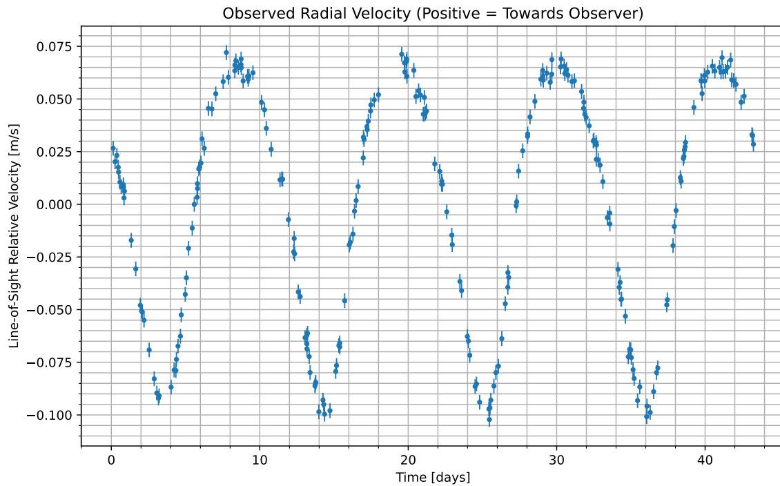
Figure 1: We have isolated the radial velocity of the host star due to the candidate planet. Data begins at UTC 2095-10-27/16:41. Positive values indicate the velocity at which the star is moving towards us; negative indicate the velocity at which it is moving away.
