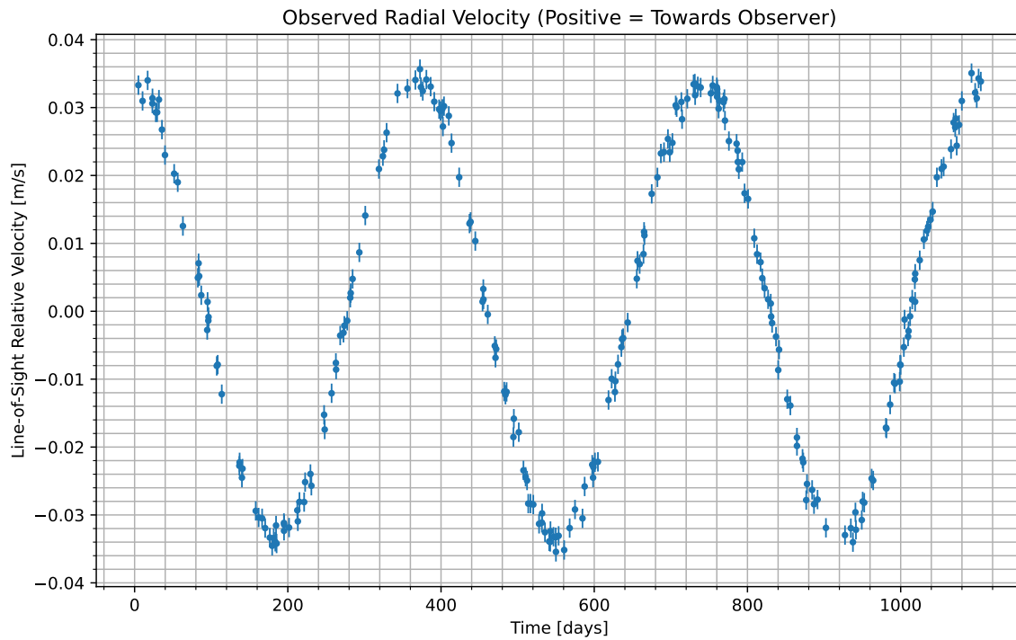
Figure 1: We have isolated the radial velocity of the host star due to the candidate planet. Data begins at UTC 2093-11-28/00:41. Positive values indicate the velocity at which the star is moving towards us; negative indicate the velocity at which it is moving away.
