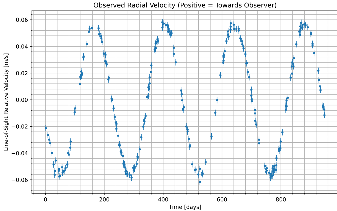
Figure 1: We have isolated the radial velocity of the host star due to the candidate planet. Data begins at UTC 2071-03-15/05:26. Positive values indicate the velocity at which the star is moving towards us; negative indicate the velocity at which it is moving away.
