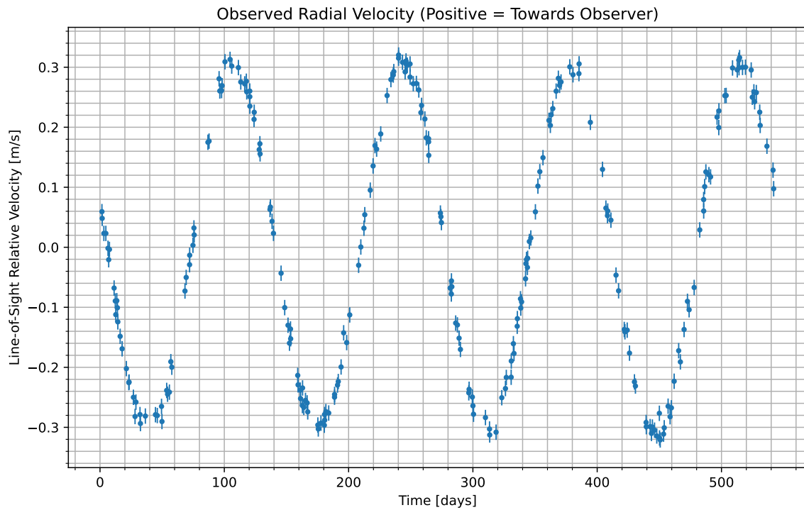
Figure 1: We have isolated the radial velocity of the host star due to the candidate planet. Data begins at UTC 2069-10-25/14:24. Positive values indicate the velocity at which the star is moving towards us; negative indicate the velocity at which it is moving away.
