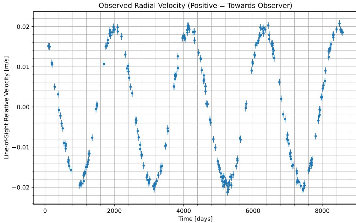
Figure 1: We have isolated the radial velocity of the host star due to the candidate planet. Data begins at UTC 2072-05-01/18:53. Positive values indicate the velocity at which the star is moving towards us; negative indicate the velocity at which it is moving away.
