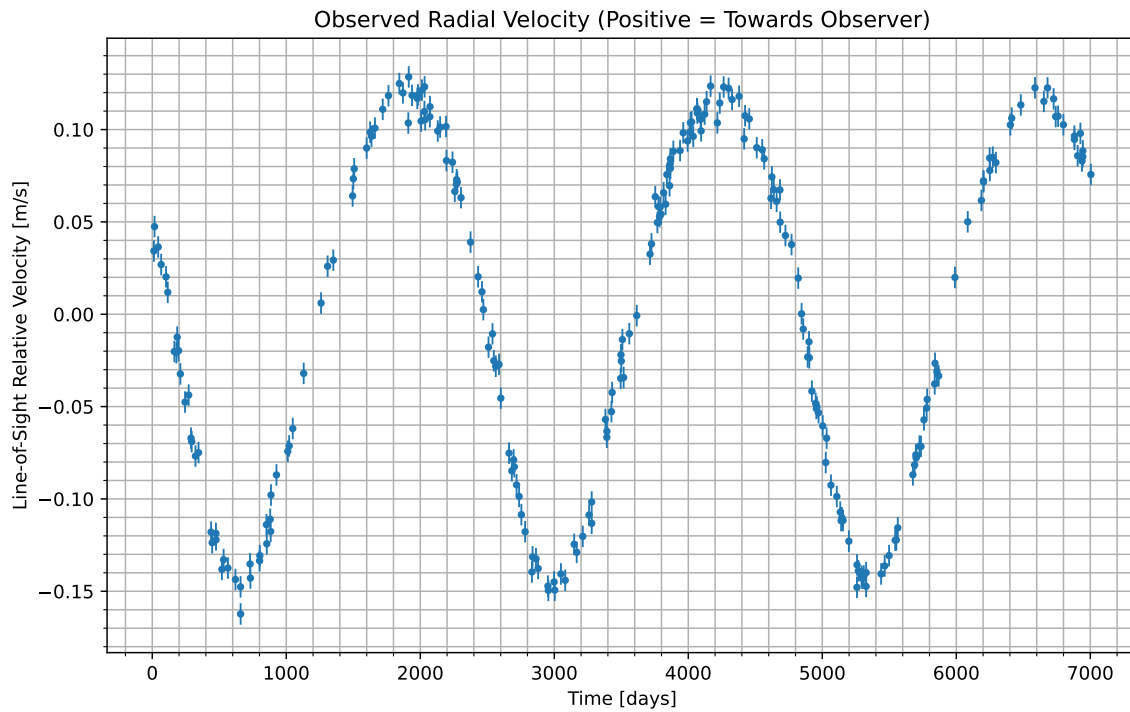
Figure 1: We have isolated the radial velocity of the host star due to the candidate planet. Data begins at UTC 2075-04-21/01:29. Positive values indicate the velocity at which the star is moving towards us; negative indicate the velocity at which it is moving away.
