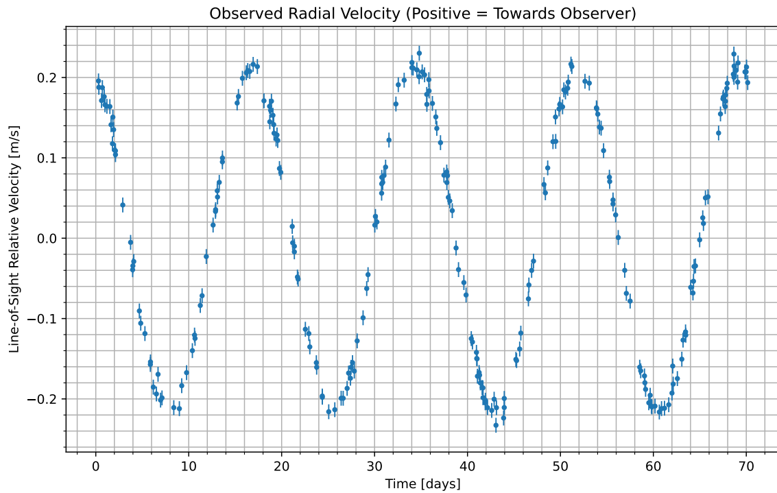
Figure 1: We have isolated the radial velocity of the host star due to the candidate planet. Data begins at UTC 2074-10-14/16:05. Positive values indicate the velocity at which the star is moving towards us; negative indicate the velocity at which it is moving away.
