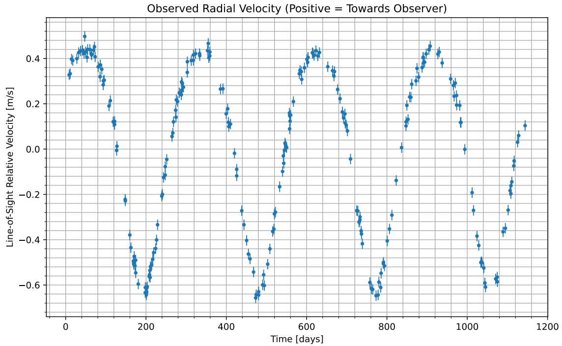
Figure 1: We have isolated the radial velocity of the host star due to the candidate planet. Data begins at UTC 2072-10-07/04:39. Positive values indicate the velocity at which the star is moving towards us; negative indicate the velocity at which it is moving away.
