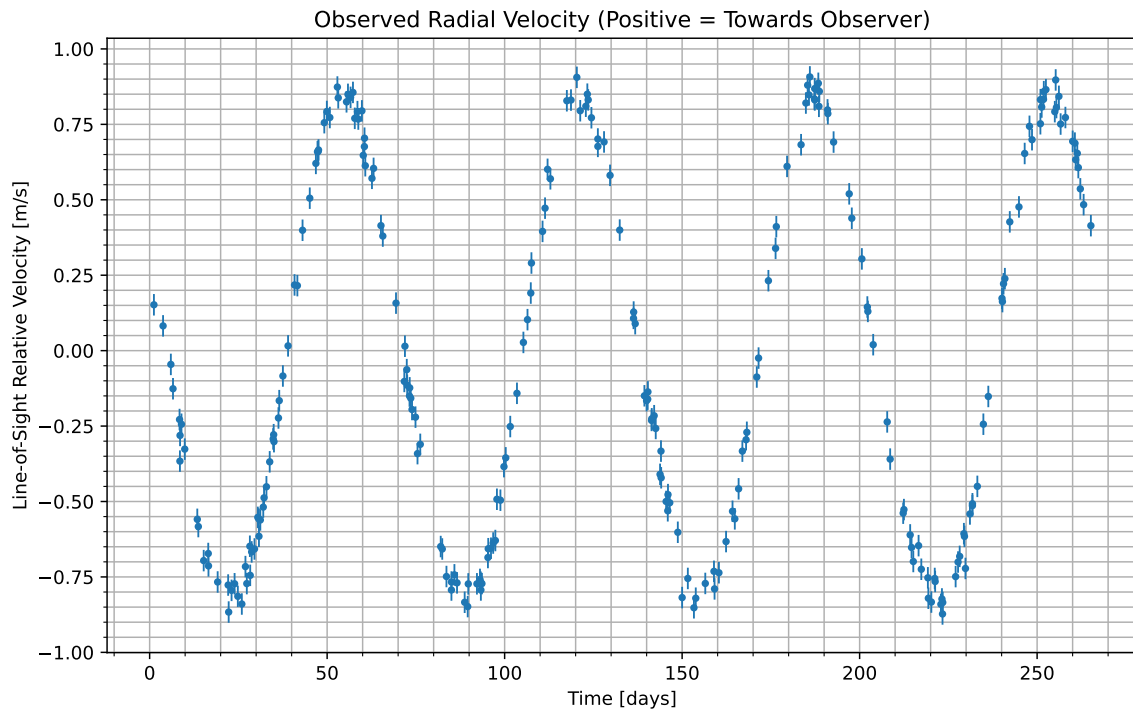
Figure 1: We have isolated the radial velocity of the host star due to the candidate planet. Data begins at UTC 2075-05-17/12:25. Positive values indicate the velocity at which the star is moving towards us; negative indicate the velocity at which it is moving away.
