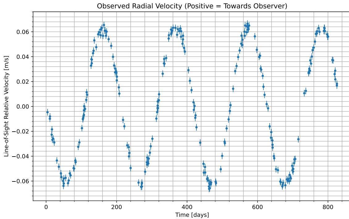
Figure 1: We have isolated the radial velocity of the host star due to the candidate planet. Data begins at UTC 2095-11-26/10:10. Positive values indicate the velocity at which the star is moving towards us; negative indicate the velocity at which it is moving away.
