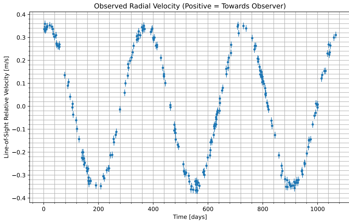
Figure 1: We have isolated the radial velocity of the host star due to the candidate planet. Data begins at UTC 2086-03-01/19:45. Positive values indicate the velocity at which the star is moving towards us; negative indicate the velocity at which it is moving away.
