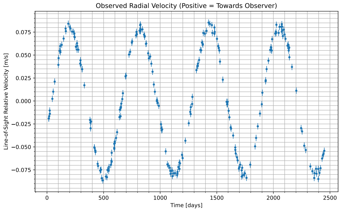
Figure 1: We have isolated the radial velocity of the host star due to the candidate planet. Data begins at UTC 2092-08-10/04:20. Positive values indicate the velocity at which the star is moving towards us; negative indicate the velocity at which it is moving away.
