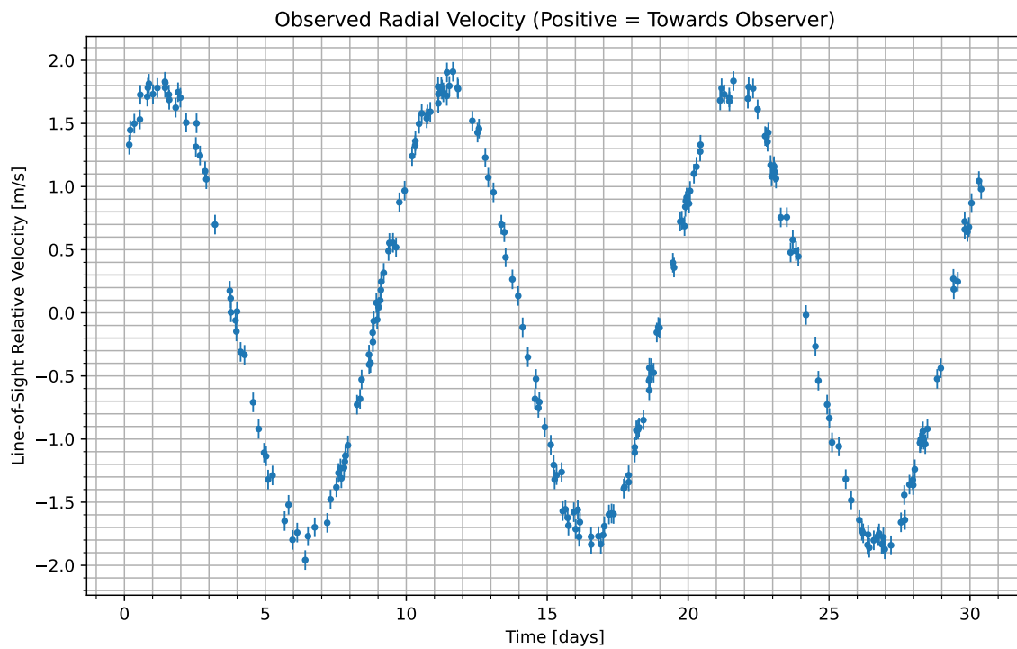
Figure 1: We have isolated the radial velocity of the host star due to the candidate planet. Data begins at UTC 2085-03-14/01:14. Positive values indicate the velocity at which the star is moving towards us; negative indicate the velocity at which it is moving away.
