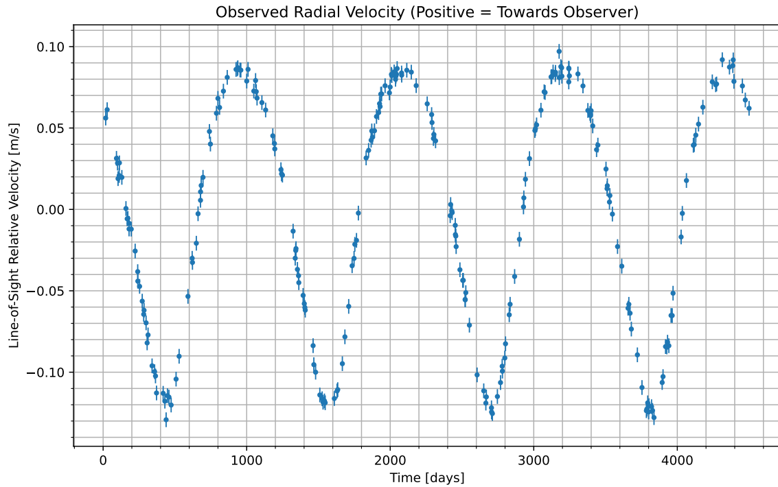
Figure 1: We have isolated the radial velocity of the host star due to the candidate planet. Data begins at UTC 2084-05-07/20:18. Positive values indicate the velocity at which the star is moving towards us; negative indicate the velocity at which it is moving away.
