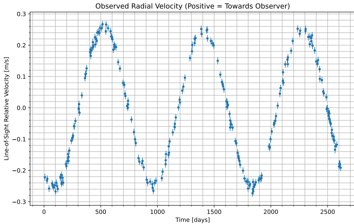
Figure 1: We have isolated the radial velocity of the host star due to the candidate planet. Data begins at UTC 2084-06-04/10:41. Positive values indicate the velocity at which the star is moving towards us; negative indicate the velocity at which it is moving away.
