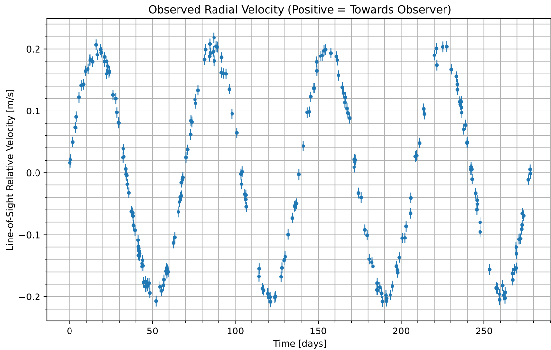
Figure 1: We have isolated the radial velocity of the host star due to the candidate planet. Data begins at UTC 2072-10-10/04:38. Positive values indicate the velocity at which the star is moving towards us; negative indicate the velocity at which it is moving away.
