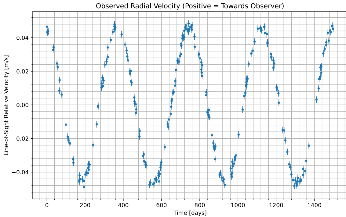
Figure 1: We have isolated the radial velocity of the host star due to the candidate planet. Data begins at UTC 2074-07-01/12:39. Positive values indicate the velocity at which the star is moving towards us; negative indicate the velocity at which it is moving away.
