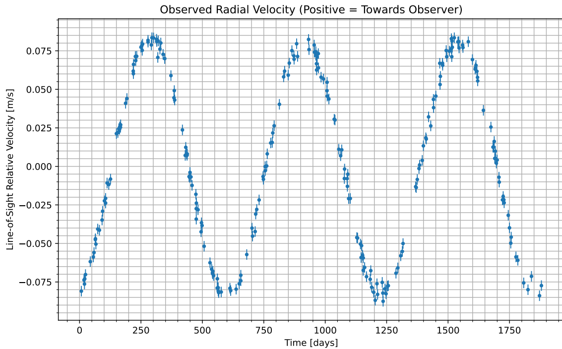
Figure 1: We have isolated the radial velocity of the host star due to the candidate planet. Data begins at UTC 2075-09-18/23:24. Positive values indicate the velocity at which the star is moving towards us; negative indicate the velocity at which it is moving away.
