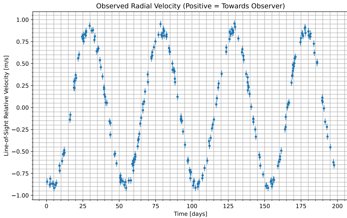
Figure 1: We have isolated the radial velocity of the host star due to the candidate planet. Data begins at UTC 2085-01-15/05:42. Positive values indicate the velocity at which the star is moving towards us; negative indicate the velocity at which it is moving away.
