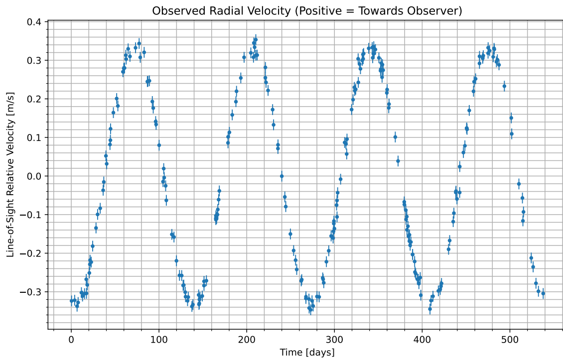
Figure 1: We have isolated the radial velocity of the host star due to the candidate planet. Data begins at UTC 2085-03-23/02:06. Positive values indicate the velocity at which the star is moving towards us; negative indicate the velocity at which it is moving away.
