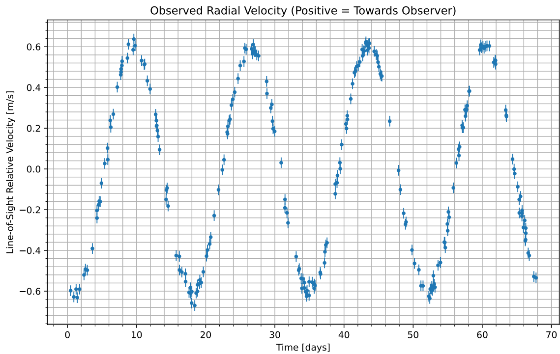
Figure 1: We have isolated the radial velocity of the host star due to the candidate planet. Data begins at UTC 2071-07-22/21:11. Positive values indicate the velocity at which the star is moving towards us; negative indicate the velocity at which it is moving away.
