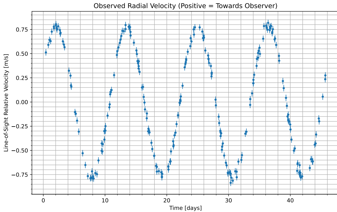
Figure 1: We have isolated the radial velocity of the host star due to the candidate planet. Data begins at UTC 2082-08-30/00:48. Positive values indicate the velocity at which the star is moving towards us; negative indicate the velocity at which it is moving away.
