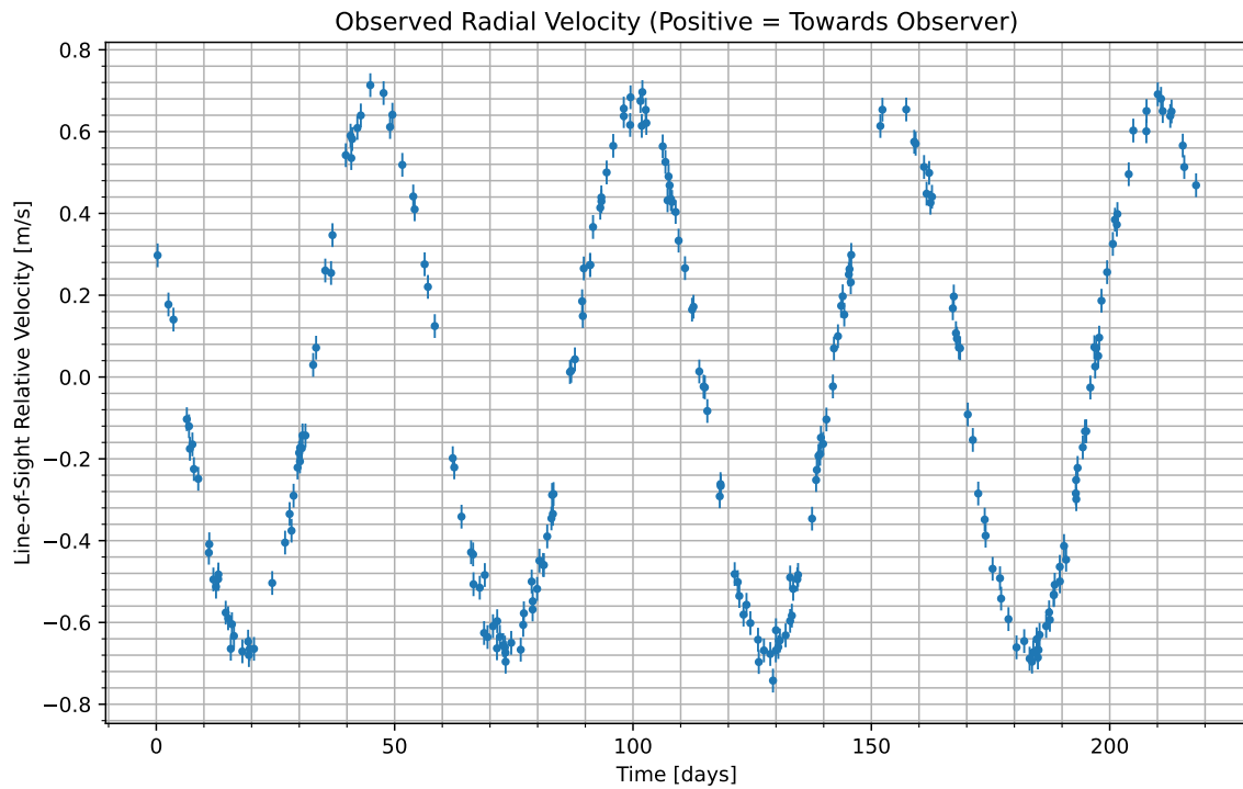
Figure 1: We have isolated the radial velocity of the host star due to the candidate planet. Data begins at UTC 2079-10-07/03:07. Positive values indicate the velocity at which the star is moving towards us; negative indicate the velocity at which it is moving away.
