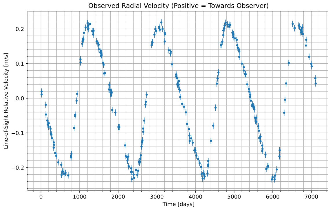
Figure 1: We have isolated the radial velocity of the host star due to the candidate planet. Data begins at UTC 2060-11-25/05:19. Positive values indicate the velocity at which the star is moving towards us; negative indicate the velocity at which it is moving away.
