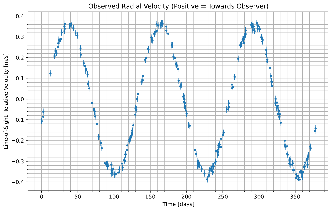
Figure 1: We have isolated the radial velocity of the host star due to the candidate planet. Data begins at UTC 2081-07-21/07:10. Positive values indicate the velocity at which the star is moving towards us; negative indicate the velocity at which it is moving away.
