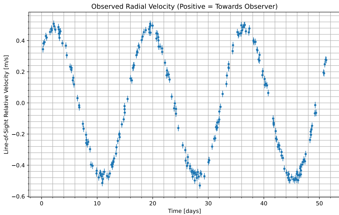
Figure 1: We have isolated the radial velocity of the host star due to the candidate planet. Data begins at UTC 2075-12-30/13:38. Positive values indicate the velocity at which the star is moving towards us; negative indicate the velocity at which it is moving away.
