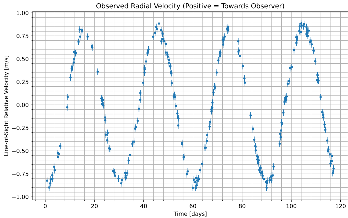
Figure 1: We have isolated the radial velocity of the host star due to the candidate planet. Data begins at UTC 2082-05-21/16:13. Positive values indicate the velocity at which the star is moving towards us; negative indicate the velocity at which it is moving away.
