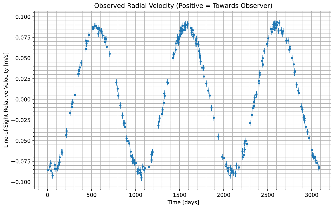
Figure 1: We have isolated the radial velocity of the host star due to the candidate planet. Data begins at UTC 2080-03-04/17:18. Positive values indicate the velocity at which the star is moving towards us; negative indicate the velocity at which it is moving away.
