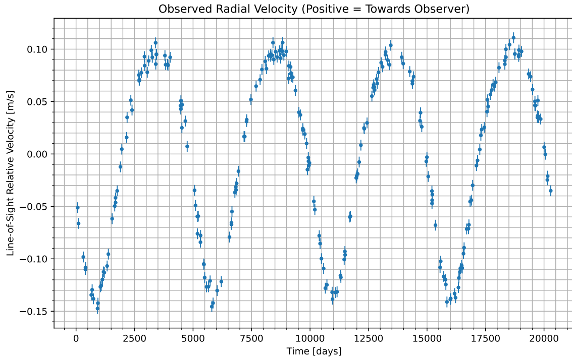
Figure 1: We have isolated the radial velocity of the host star due to the candidate planet. Data begins at UTC 2034-05-31/19:16. Positive values indicate the velocity at which the star is moving towards us; negative indicate the velocity at which it is moving away.
