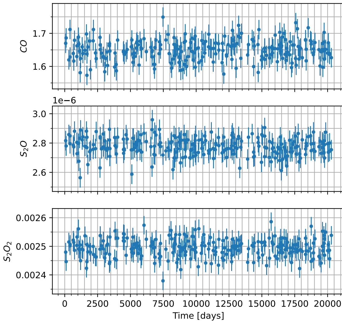
Figure 4: Concentration of various additional gases in the atmosphere of the candidate planet versus time. Note that the y-axis will usually only show the variation multiplied by some factor, shown in the upper left, and then added to some normal amount, also in the upper-left.
