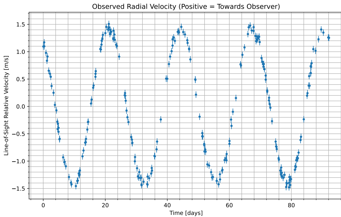
Figure 1: We have isolated the radial velocity of the host star due to the candidate planet. Data begins at UTC 2100-04-03/20:53. Positive values indicate the velocity at which the star is moving towards us; negative indicate the velocity at which it is moving away.
